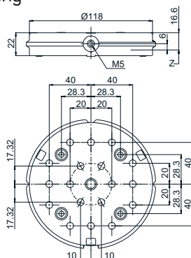
/// Pallet with coined cams
